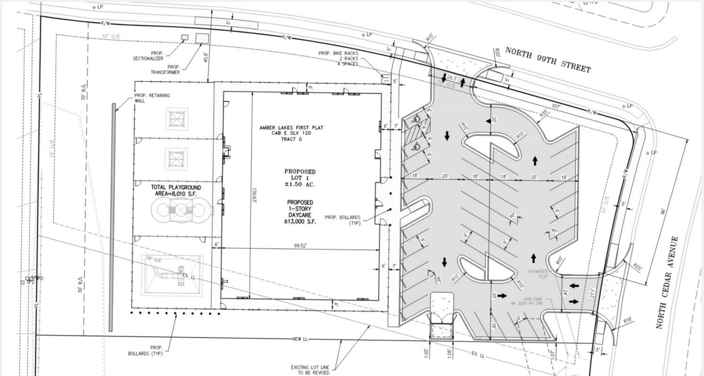
Site Plan
