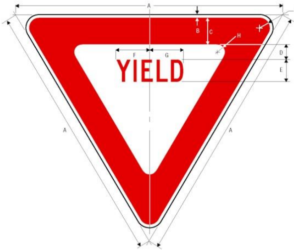
R1-2 YIELD
