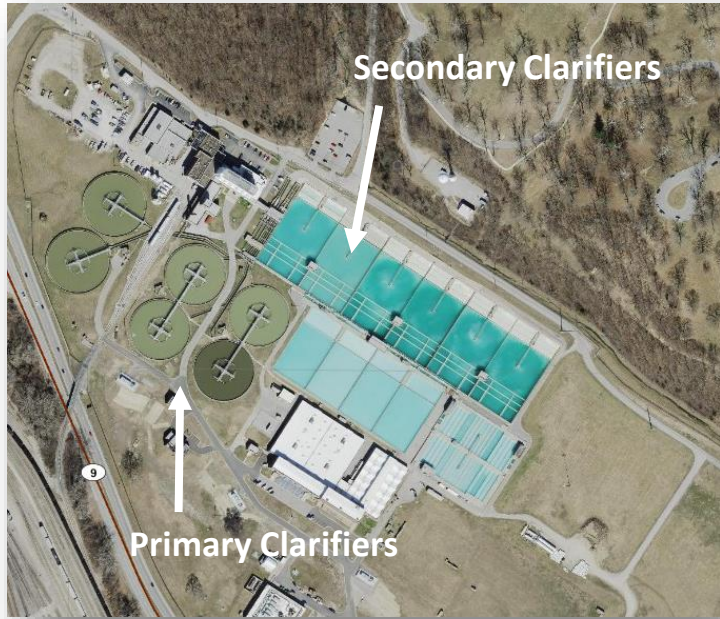
Water Treatment Plant Primary and Secondary Clarifiers and Secondary Basins
