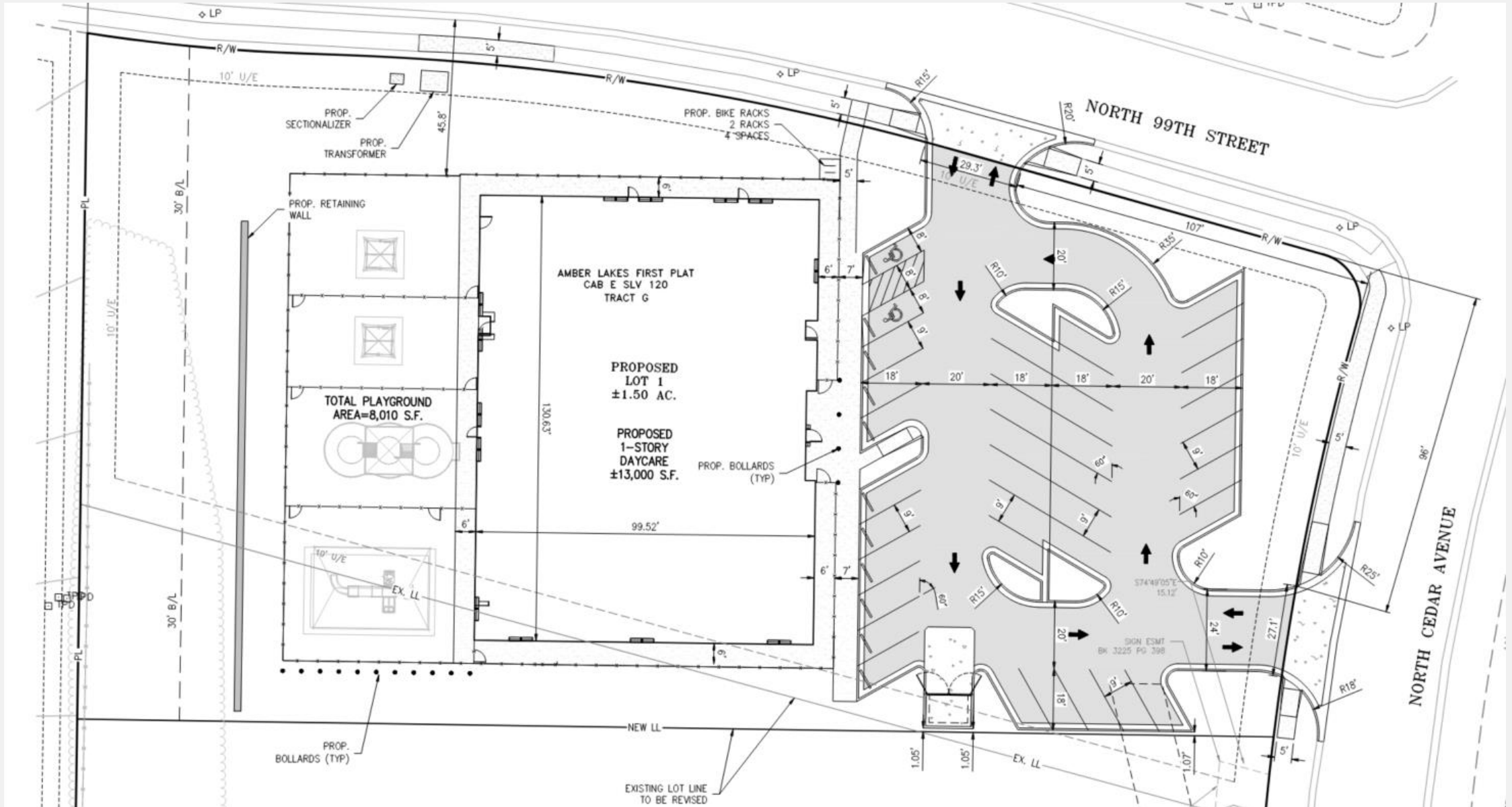
Site Plan
