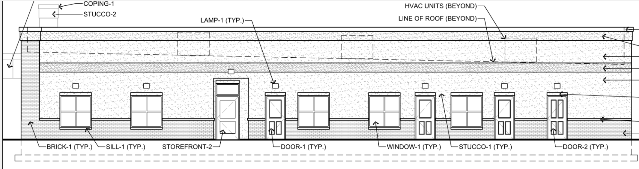
North Elevation
