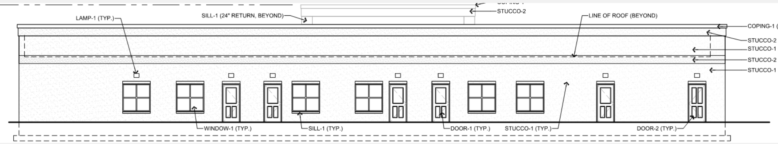
West Elevation (facing playground)
