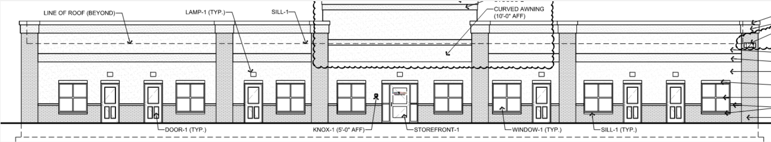
East Elevation (front)
