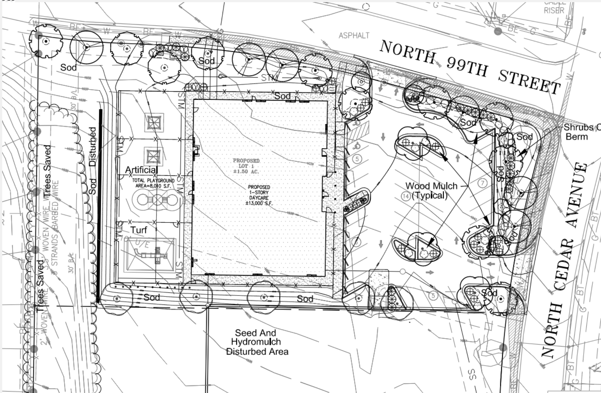
Landscape Plan
