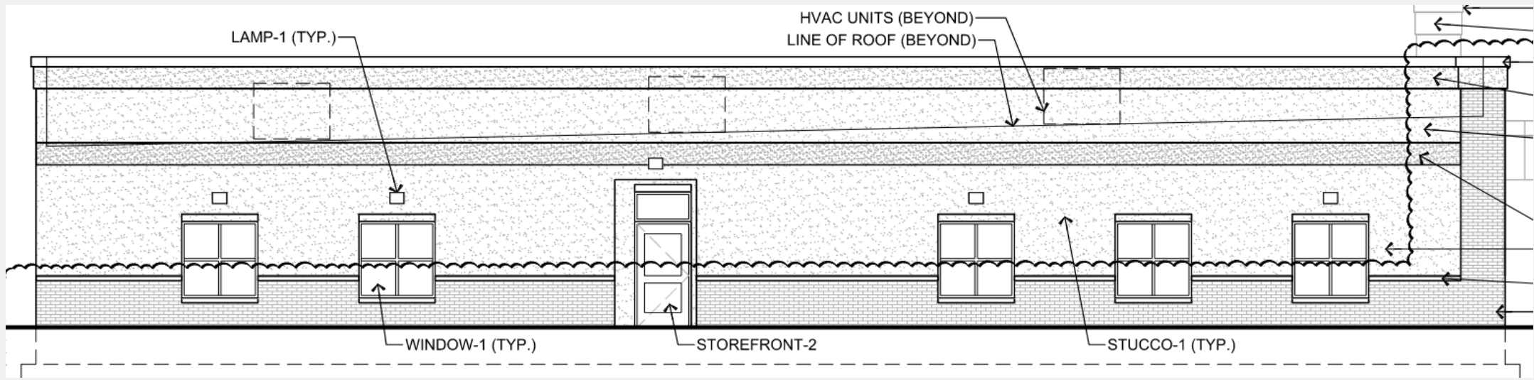
South Elevation
