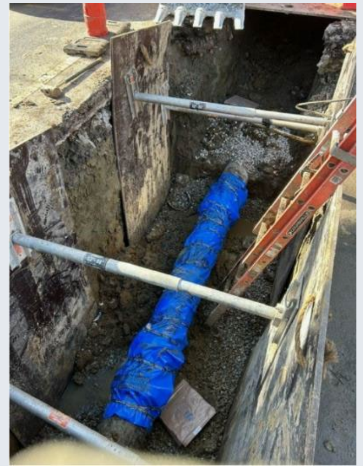
Replacement of a Cast Iron with Ductile Iron Pipe
