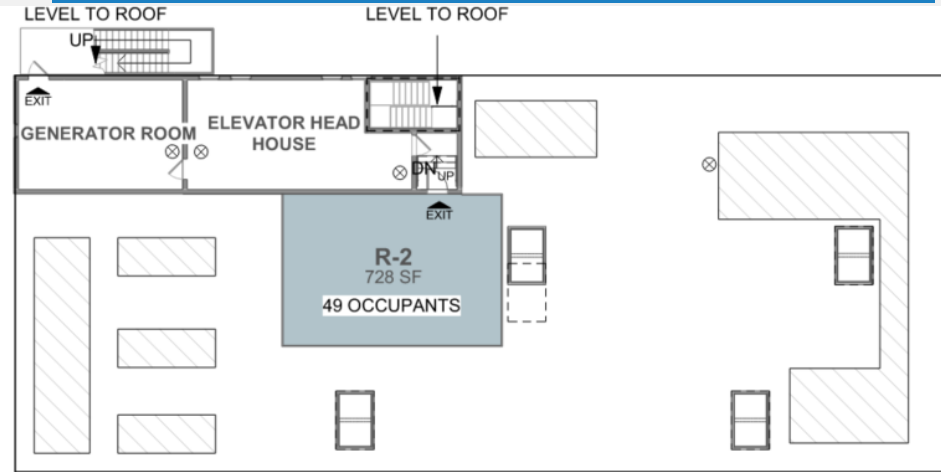
7 | ROOF - CODE PLAN 1" = 20'-0"
