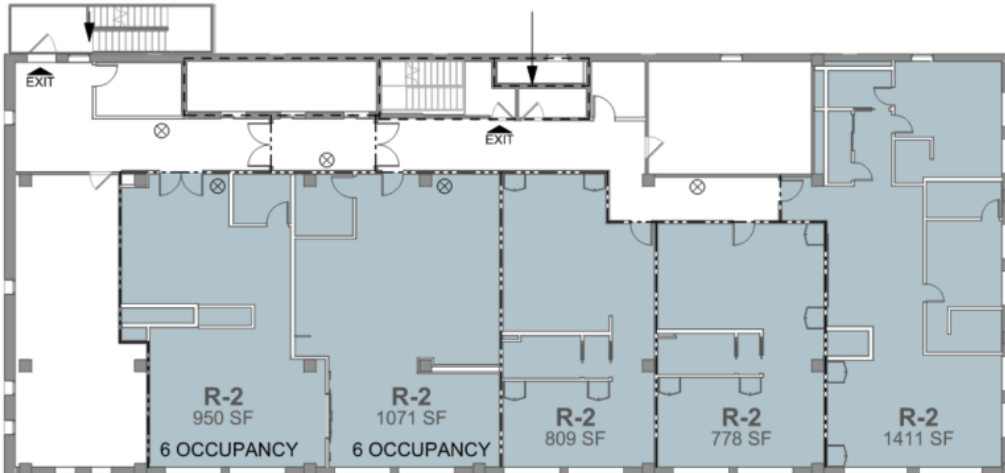
6 | 11_ELEVENTH FLOOR 1" = 20'-0"
