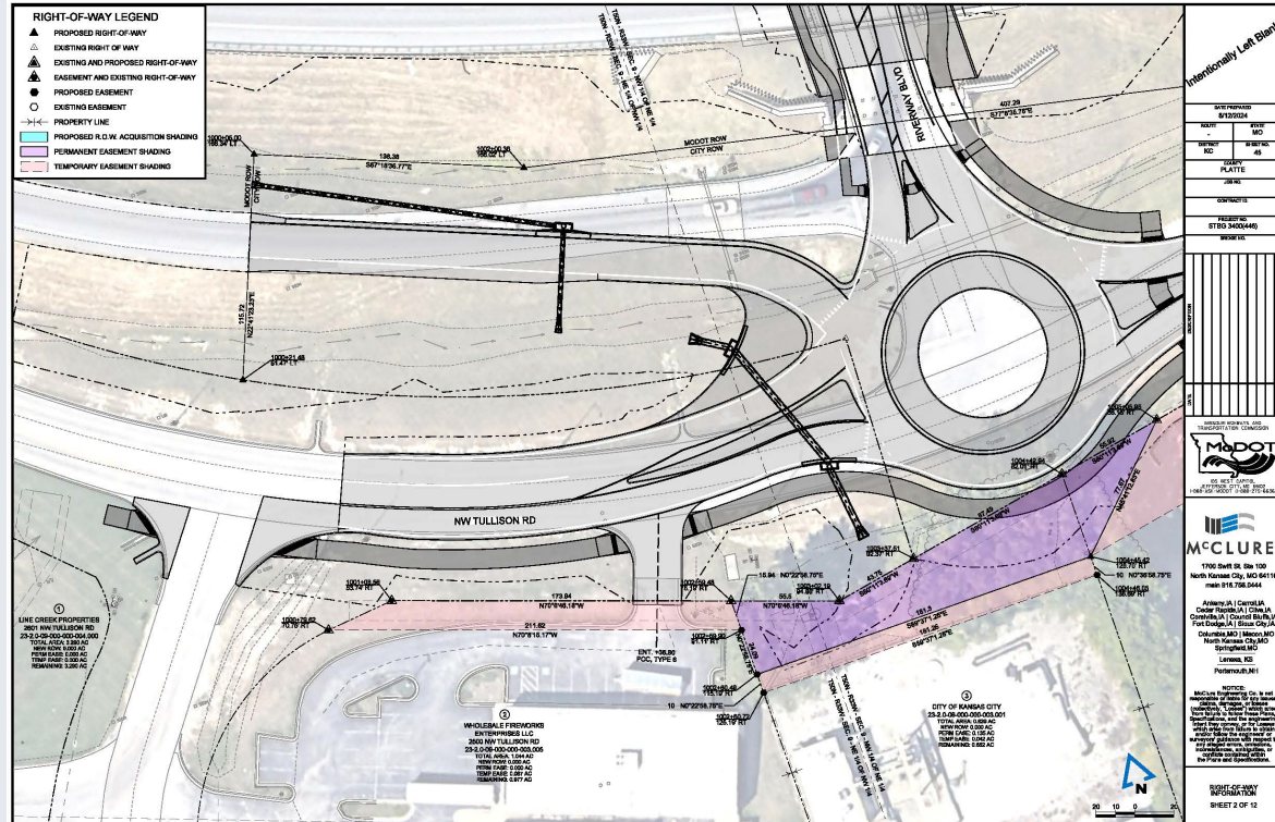
Northwest Tullison Road Project Right of Way Plan Sheet
