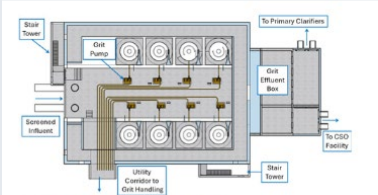
Figure 1.19 Grit Alternative No. 2 – New Grit Facility Lower Level Plan View
