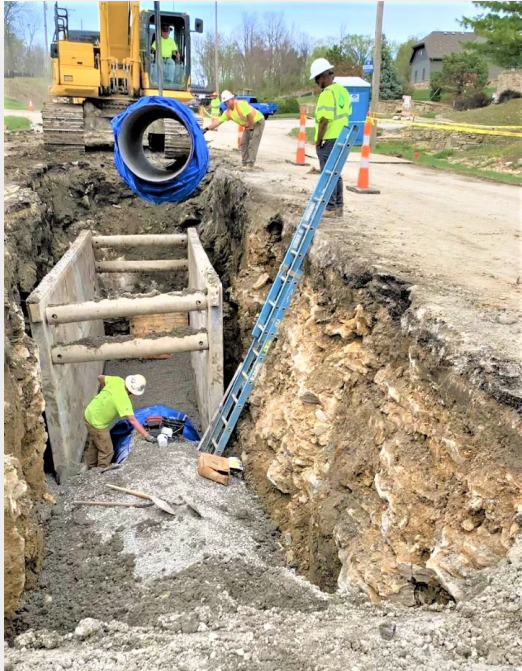
Crew lowering a pipe section to install a water main replacement.
