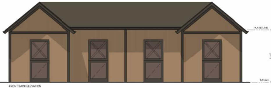
FUTURE ACCESSORY BARN CONCEPT ELEVATIONS 1/4" = 1'-0"
