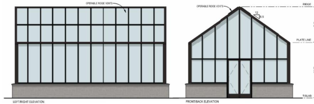
FUTURE GREENHOUSE CONCEPT ELEVATIONS 1/4" = 1'-0"
